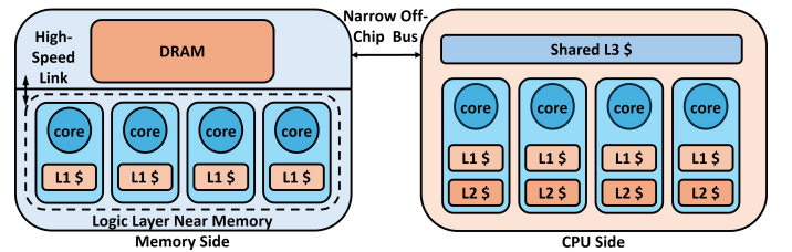
Fig. 3. A high-level CPU-NDP architecture.
